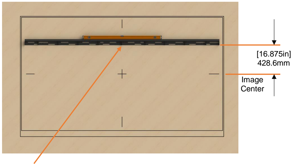
Mount bar centerline
