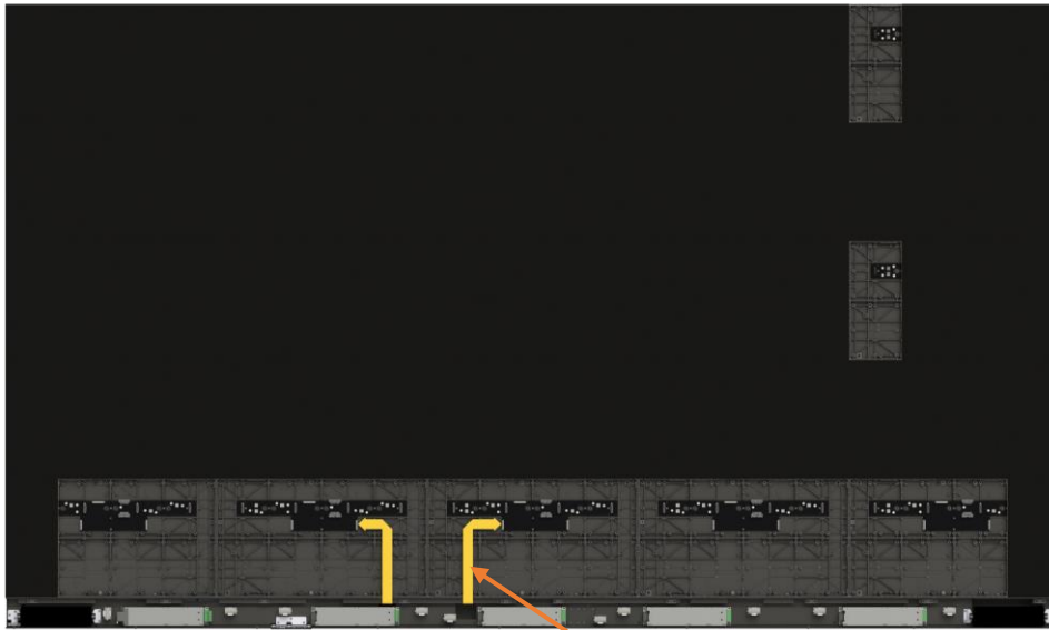
2X Flat Flex Cables
